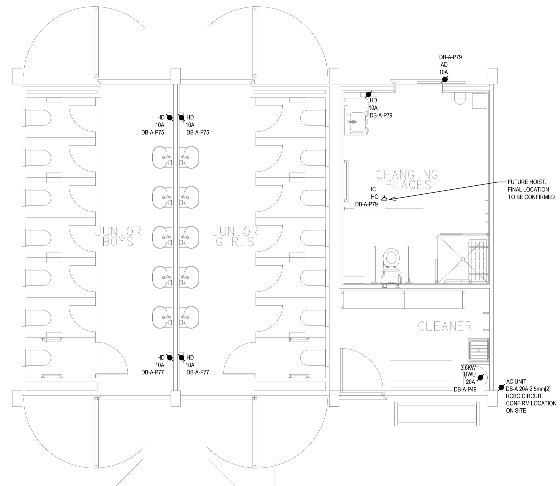
PROPOSED POWER & COMMUNICATIONS LAYOUT JUNIOR STUDENTS SCALE 1: 50
