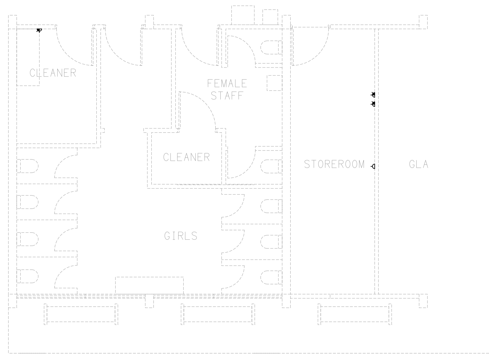
EXISTING / DEMOLITION POWER & COMMUNICATIONS LAYOUT SCALE 1: 50
